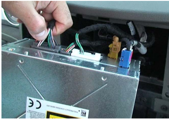
PLUG GRAY CONNECTOR FROM MYGIG LOCKPICK V.4 HARNESS INTO LOCATION SHOWN
