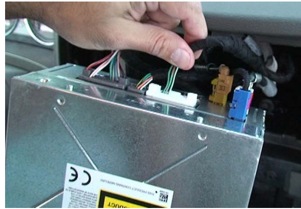
PLUG WHITE CONNECTOR FROM MYGIG LOCKPICK V.4 HARNESS INTO LOCATION SHOWN
